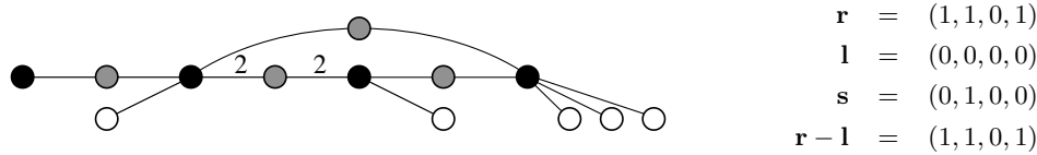
Fig. 3: The result of applying Steps 1-3 to Figure 2.
