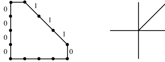
Fig. 8: The first-quadrant polygon \Delta((1, 0), (1; 3, 1)) and its normal fan.
