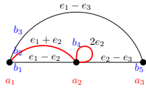
Fig. 1: A signed graph G on three vertices and the roots associated with each edge. The Kostant partition function K_G(\mathbf{a}) counts the number of ways of obtaining \mathbf{a} as a nonnegative integer combination of the roots associated to G .
