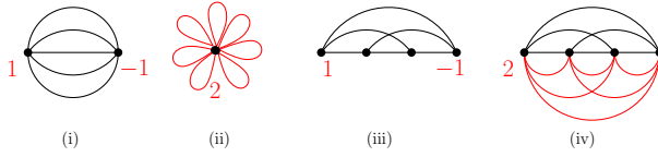
Fig. 4: Graphs whose flow polytopes are: (i) and (ii) are simplices and (iii),(iv),(v) give instances of CRYA_n , CRYD_n and CRYC_n .
