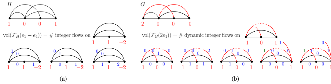
Fig. 8: Examples of Theorems 1 and 2. (a) Given a graph H with negative edges then \text{vol}(\mathcal{F}_H(1, 0, 0, -1)) = K_H(0, 1, 1, -2) = 3 this is \#\{\text{integer flows on } H \text{ excess flow } (0, d_2, d_3, d_4) = (0, 1, 1, -2)\} . (b) Given signed graph G then \text{vol}(\mathcal{F}_G(2, 0, 0, 0)) = K_G^{\text{dyn}}(0, 1, 0, 1) = 5 this is \#\{\text{dynamic integer flows on } G \text{ with excess flow } (0, d_2, d_3, d_4) = (0, 1, 0, 1)\} .
