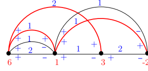
Fig. 2: A nonnegative integer flow on a signed graph G with excess flow vector \mathbf{a} = (6, 1, 3, -2) . The flows on the edges are in blue. The + and - signs denote the sign of the incidences of the edges.
