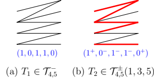
Fig. 5: Examples of bipartite non-crossing trees.
