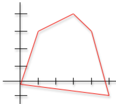
Fig. 1: A Newton polygon in GL_5(F) .
