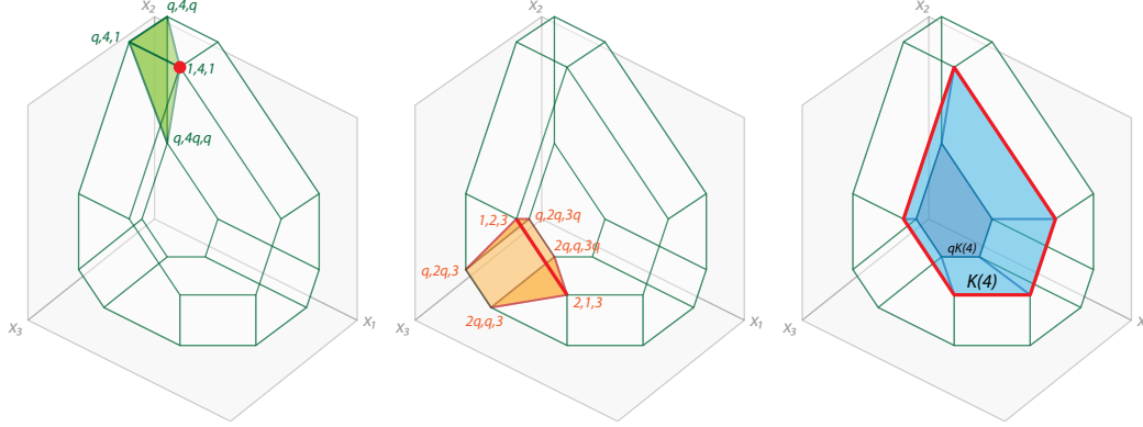
Fig. 7: Three face q -liftings of the associahedron \mathcal{K}(4) : \mathcal{K}(4)^{1|3|2}(q) , \mathcal{K}(4)^{12|3}(q) , and \mathcal{K}(4)^{123}(q) . The red regions represent the faces \mathcal{K}(4)_\pi .
