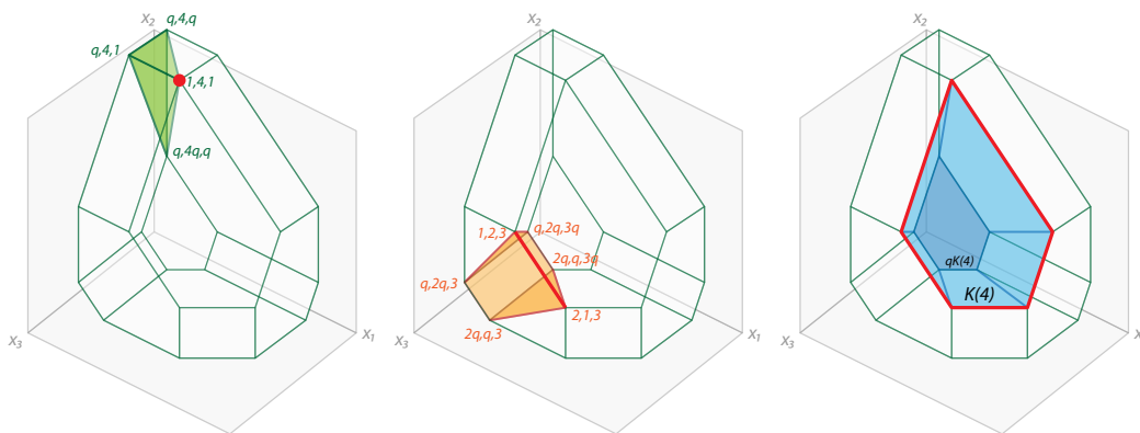
Fig. 7: Three face q -liftings of the associahedron \mathcal{K}(4) : \mathcal{K}(4)^{1|3|2}(q) , \mathcal{K}(4)^{1,2|3}(q) , and \mathcal{K}(4)^{123}(q) . The red regions represent the faces \mathcal{K}(4)_\pi .
