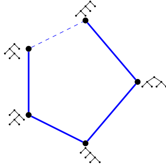
Fig. 1: The comb poset \mathcal{C}_4
