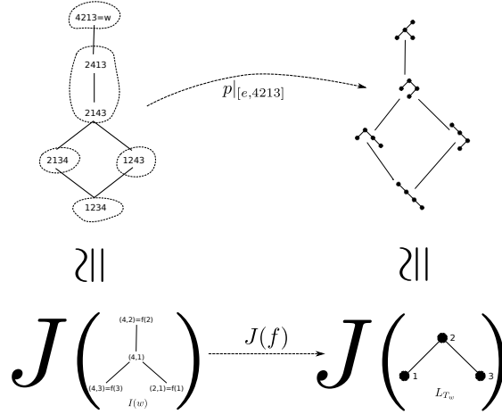
Fig. 10: p|_{[e, 4213]} and J(f) for the interval [e, 4213]_{\mathcal{C}_n} .
