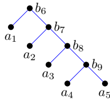
Fig. 4: RightCombTree(5)
