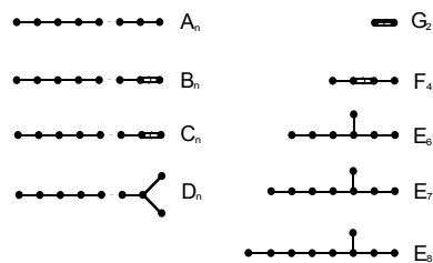
Fig. 7: Simple Dynkin diagrams
