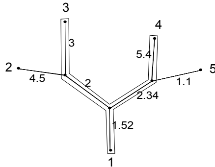
Fig. 3: d_{134}(T, w) = 14.26
