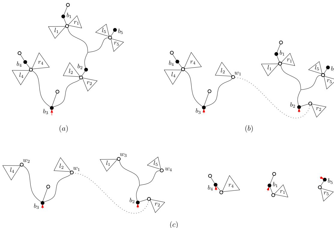
Fig. 2: From a bipartite mobile with 5 marked black vertices to a forest with 5 connected components and 4 marked white vertices \{w_1, w_2, w_3, w_4\} : (a) removing the buds on marked black vertices, (b) cutting the mobile at a marked black vertex into two connected components ( 5 - 1 choices) and a marked white vertex w_1 , (c) repeating the same operation 3 more time to obtain 5 connected components and 4 marked white vertices.
