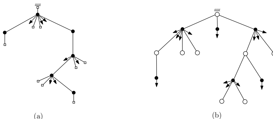
Fig. 3: (a) A blossoming tree. (b) The corresponding rooted bipartite mobile.
