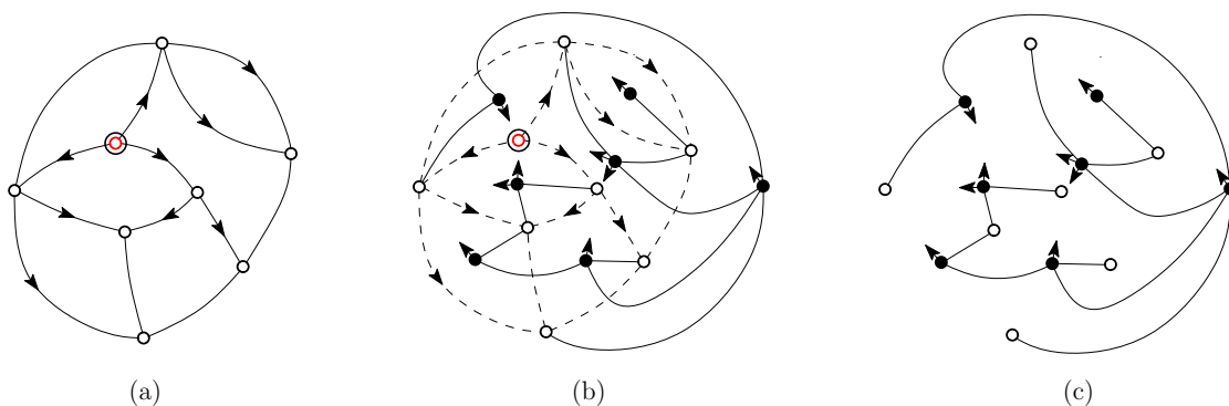
Fig. 1: (a) A vertex-pointed map endowed with the geodesic orientation (with respect to the marked vertex). (b) The local rule is applied to each edge of the map. (c) The resulting mobile.
