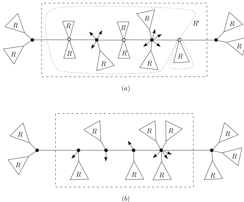
Fig. 4: middle-parts in the bipartite case (a) and in the quasi-bipartite case (b).
