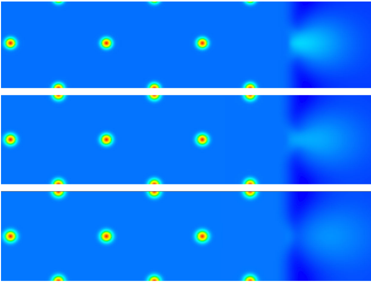
Fig. 2 Fuel mass fraction at three instants after ignition (alkane-air spray: \varphi_T = 1.2 , \varphi_G = 0.7 , \varphi_L = 0.5 , s = 6 )
