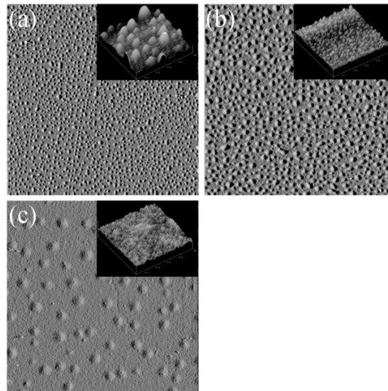
Fig.5. Surface morphology of \text{Fe}_{35}\text{Co}_{65} films evaporated on Si (100) for different thicknesses (a) t=9 nm, (b) t= 20 nm, (c) t=50 nm, obtained by AFM scan over 10\mu\text{m} \times 10\mu\text{m} surface. The insert of fig. 5 show a 3D plot of a 1\mu\text{m} \times 1\mu\text{m} zoom.
