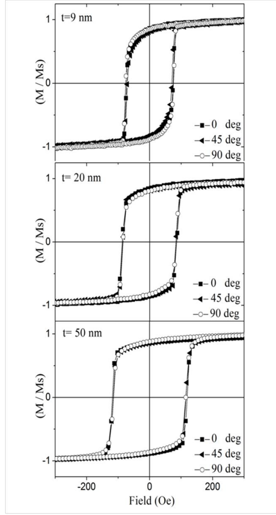
Fig.7. VSM measurement of Fe 35 Co 65 respectively 9nm, 20nm and 50nm thick. For each samples, magnetization is recorded along three different direction of magnetic field 0°, 45° and 90° relative to the (110) direction of the Si substrate.
