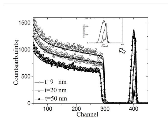
Fig. 3. RBS energy spectra collected at 165^\circ for \text{Fe}_{35}\text{Co}_{65} films deposited on silicon substrate, using 2 MeV alpha particles. Solid lines correspond to fitted spectra. Insert of fig. 3 represents a zoom of the peaks corresponding to backscattered alpha particles from Fe and Co atoms
