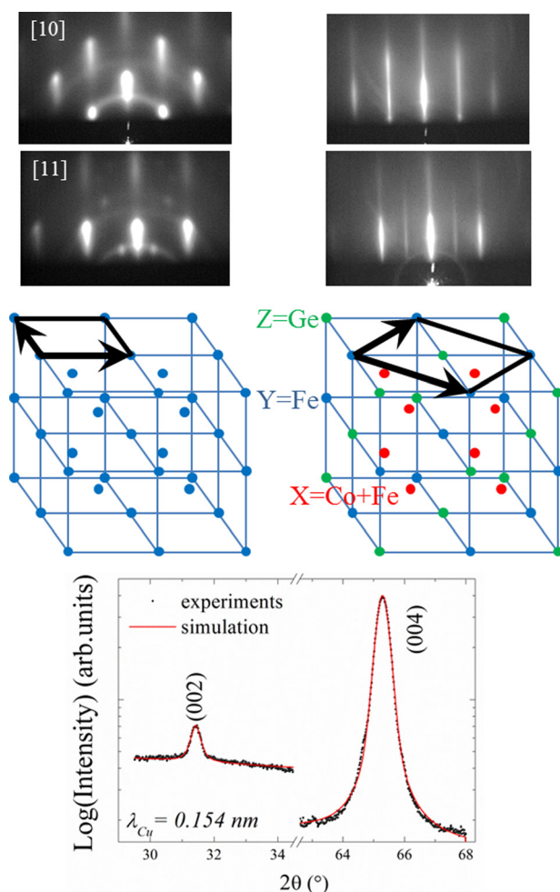
FIG. 1. RHEED patterns obtained on a CFG film as-deposited at RT (top left) and annealed (top right). New \frac{1}{2} streaks appear after annealing typical of chemical ordering. The (00L) diffraction peak intensities are also well fitted assuming the full Heusler \text{L}_{21} structure (bottom).
