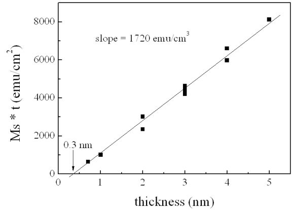
Fig. 3. Areal magnetization versus Fe thickness. The linear fit has positive slope value 1720 emu/cm 3 . It crosses zero areal moment for a non-zero-thickness meaning that Fe magnetization is reduced in average over about 2 atomic layers.
