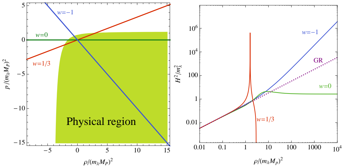
Figure 1. Left panel: Region in the plane (\bar{\rho}, \bar{P}) obtained by imposing that the fundamental matrix \hat{M} is positive definite, i.e., that both M_0 and M_1 are real and positive valued. We see that such a region is basically defined by the simultaneous conditions \rho \gtrsim -4m_\lambda^2 M_{\text{Pl}}^2 and \bar{P} \lesssim m_\lambda^2 M_{\text{Pl}}^2 . For an idealized barotropic fluid P = w\rho , with a constant equation of state parameter w , the pressure and/or the energy densities may end up being bounded. Right panel: We show the Hubble function as a function of the energy density for different equation of state parameters illustrating the 3 behaviours discussed in the main text. We can see that at low energy densities they all follow the usual GR behavior (dotted line), whereas at high energy densities ( \rho \gg m_\lambda^2 M_{\text{Pl}}^2 ) the differences appear. In particular, for a dust component with w = 0 we see that H^2 goes to a constant value, i.e., it gives a de Sitter phase.
