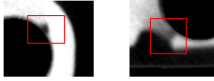
Figure 3. Part of a slice view extracted from a 3D-CT volume: on the left side a true defect (surface defect) appears as a darker area and on the right side a false alarm (reconstruction artefact) appears as a darker area as well.
