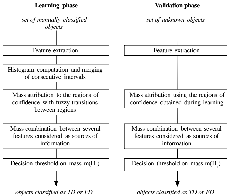
Figure 1. Flow diagram of the proposed Data Fusion Classification method.
