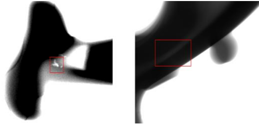
Figure 2. Inside the left side red rectangle appears a true defect and on the right side red rectangle appears an artefact caused by the structure of the inspected part.
