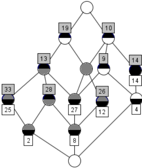
Figure 4: A lattice with its irreducible nodes. Nodes with a number above are meet-irreducible while nodes with a number below are join-irreducible.
