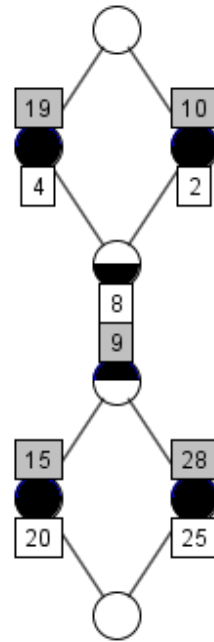
Figure 3: The lattice of congruence relations of the lattice given in Figure 2
