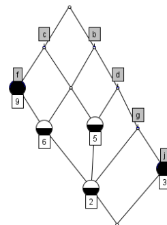
Figure 1: A lattice with its irreducible nodes
