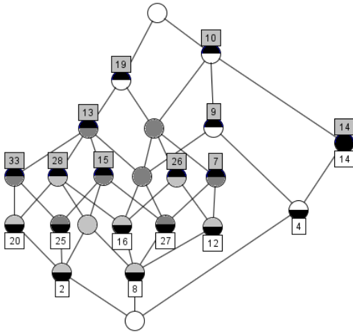
Figure 2: The lattice of Figure 4 with the convex set doubled. Nodes of each convex are colored in light grey and dark grey.
