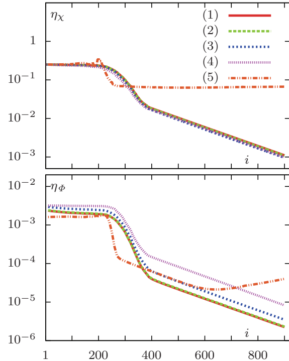
FIG. 3. Convergence data for the small target. Errors \eta_\chi and \eta_\phi are plotted vs the iteration number i . Different line types correspond to different contrast \chi_0 as follows: \chi_0 = 0.00175 (1), \chi_0 = 0.0175 (2), \chi_0 = 0.175 (3), \chi_0 = 0.875 (4), and \chi_0 = 1.75 (5).
