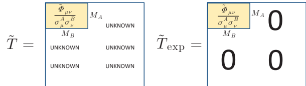
FIG. 3. (color online) Left panel: Elements of \tilde{T} inside the shaded block can be computed from the data by using (17). Elements outside of the shaded block are not known and can not be in any way inferred from the data. Right panel: The initial guess for the T-matrix, T_{\text{exp}} . In this initial guess, we set the unknown elements of \tilde{T} (in singular-vector representation) to zero.
