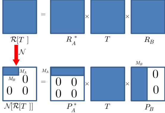
FIG. 6. (color online) Schematics of computing \mathcal{N}[\mathcal{R}[T]] . Matrices P_A and P_B are obtained from R_A and R_B by setting all columns to zero except for the first M_A and M_B columns, respectively.
