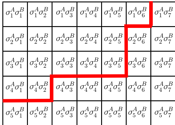
FIG. 4. (color online) Assuming that the singular values \sigma_\mu^A and \sigma_\nu^B are arranged in the descending order, this sketch shows an example of a more general shape (compared to Fig. 3) of the region in which the elements of \tilde{T} are known. The numbers above the thick line satisfy \sigma_\mu^A \sigma_\nu^B > \epsilon^2 . In the general case, the boundary line can only go from left to right and from bottom to top if followed from the left-most boundary of the matrix.
