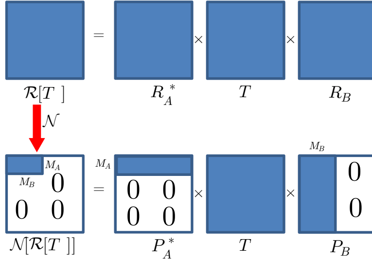
Figure 6. (color online) Schematics of computing \mathcal{N}[\mathcal{R}[T]] . Matrices P_A and P_B are obtained from R_A and R_B by setting all columns to zero except for the first M_A and M_B columns, respectively.
