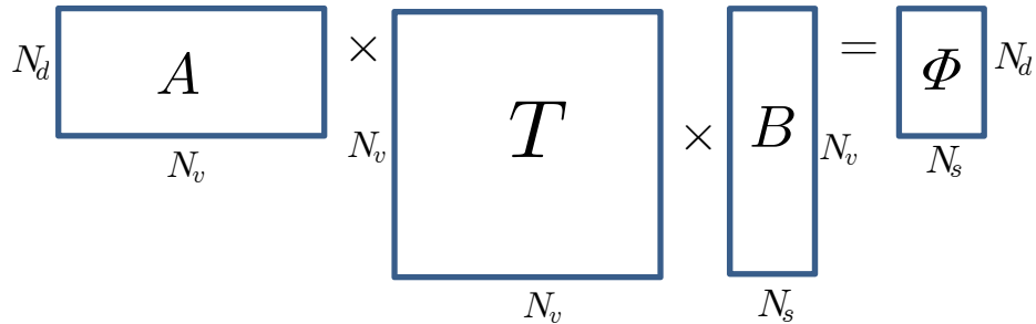
Figure 2. (color online) Block diagram of Eq. (8) with sizes of all matrices indicated. here N_d and N_s are the numbers of detectors and sources and N_v is the number of voxels.
