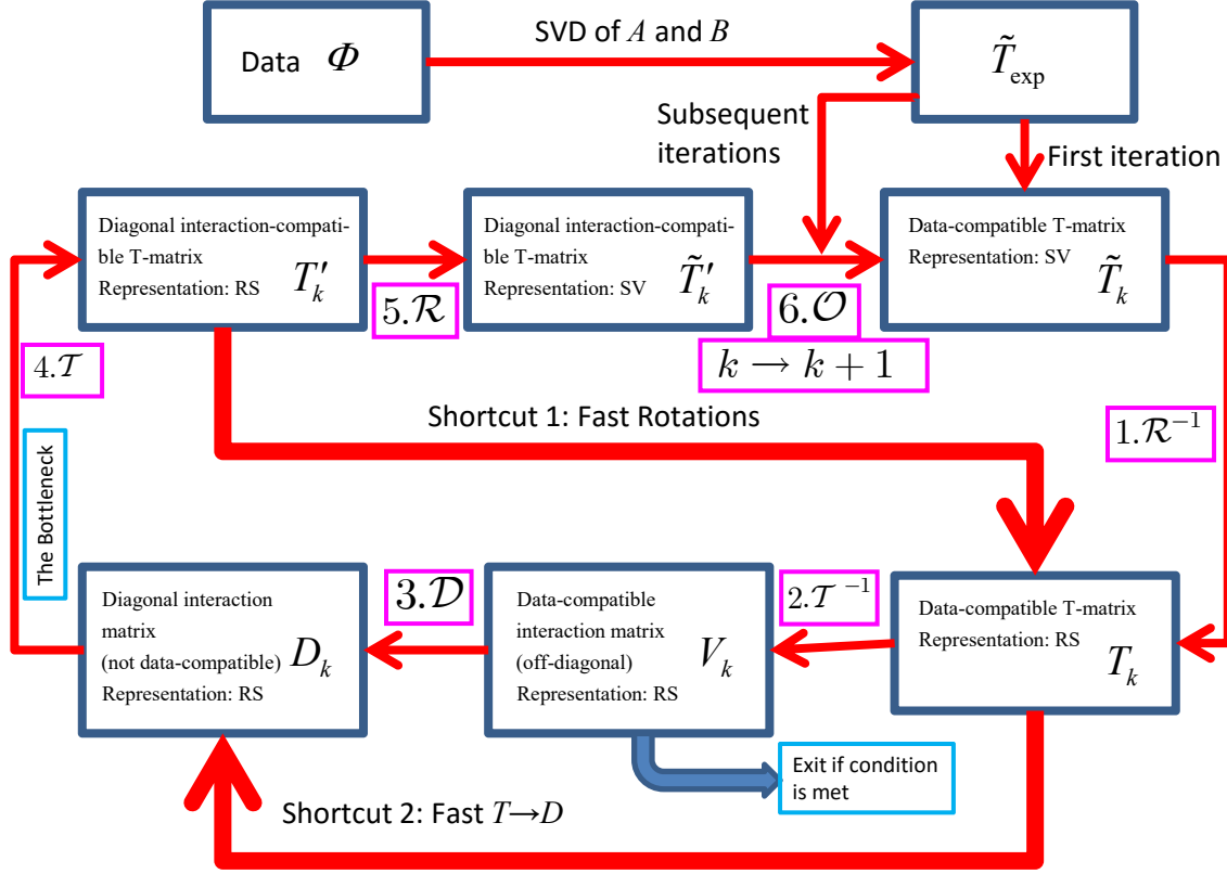
Figure 5. (color online) Basic flowchart of the DCTMC iteration process for the case when the iterations start with an initial guess for \tilde{T} . Other options are discussed in Sec. 6.1. Numbered iteration steps are defined in Sec. 4. Computational shortcuts are described in Sec. 5. The iteration step labeled "The Bottleneck" is the step in comparison to which the complexity of all other steps can be made insignificant. Eliminating the bottleneck by accounting for sparsity of V is discussed in Sec. 6.2. Matrix representations are abbreviated by SV (singular-vector) and RS (real-space).
