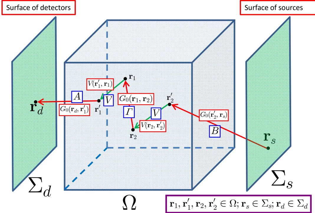
Figure 1. (color online) Illustration of the imaging geometry. The symbols A , B , \Gamma and V in blue frames denote the matrices obtained by restricting and sampling the kernels G_0(\mathbf{r}, \mathbf{r}') and V(\mathbf{r}, \mathbf{r}') . The scattering diagram corresponds to the second order term G_0 V G_0 V G_0 in the formal power-series expansion of the left-hand side in (3). Note that in the local limit V(\mathbf{r}, \mathbf{r}') = D(\mathbf{r})\delta(\mathbf{r} - \mathbf{r}') , the two green arrows contract to two vertexes at \mathbf{r}_1 = \mathbf{r}'_1 and \mathbf{r}_2 = \mathbf{r}'_2 .
