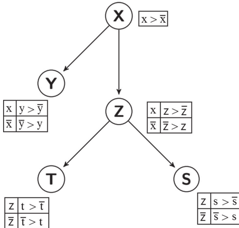
Fig. 1 CP-net associated to Example 1
