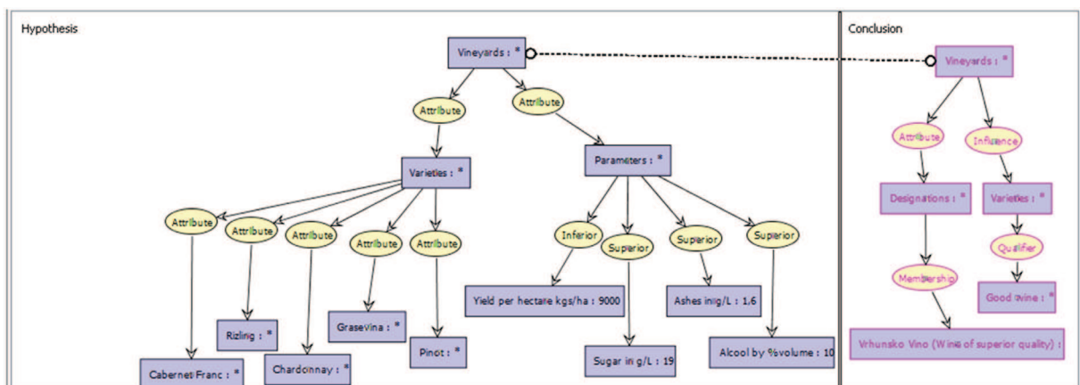
Fig. 8. An example of graph rules (Vrhunsko Vино region B).
