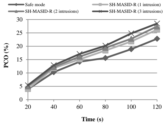
Figure 2. Protocol control overhead vs. time
