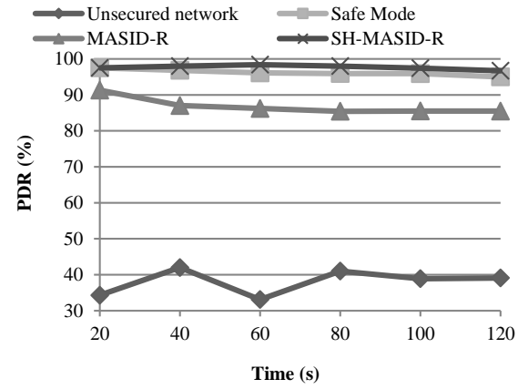
Figure 1. Packet delivery ratio vs. time
