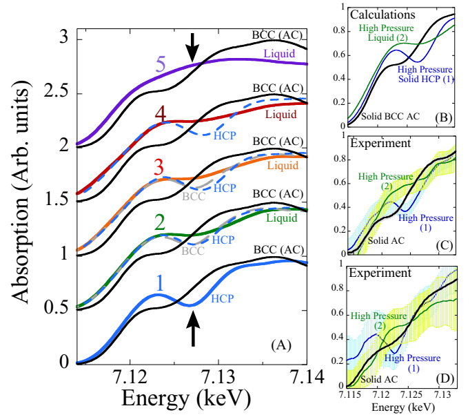
FIG. 6. (Color online) (a) Ab initio calculated XANES spectra of liquid Fe (full lines), hcp, and bcc Fe (dotted lines) phases compared to solid bcc Fe at ambient conditions (AC) (black lines). XANES spectra are calculated at the same temperatures and pressures than of the experimental groups, labeled from 1 to 5 (see Fig. 3) with (1) 11.25 g/cc-2780 K-130 GPa, (2) 12.45 g/cc-5680 K-260 GPa, (3) 13.5 g/cc-8120 K-380 GPa, (4) 13.8 g/cc-10 800 K-420 GPa, and (5) 6 g/cc-4180 K-12 GPa. (b) Zoom of the pre-edge region of the calculated XANES spectra of bcc iron at ambient conditions AC (black line), solid hcp Fe at 130 GPa (blue line), and liquid Fe at 260 GPa (green line). (c) Experimental XANES spectra obtained with the Si crystal spectrometers diagnostic at the same conditions. (d) Experimental XANES spectra obtained with the quartz spectrometer at similar conditions.
