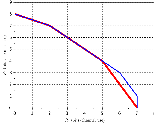
Figure 4: Capacity regions \mathcal{C}(0,0) (thick red line) and \mathcal{C}(0,7) (thin blue line), with \overleftarrow{n}_{11} = 7 , \overleftarrow{n}_{22} = 8 , n_{12} = 6 , n_{21} = 5 .
