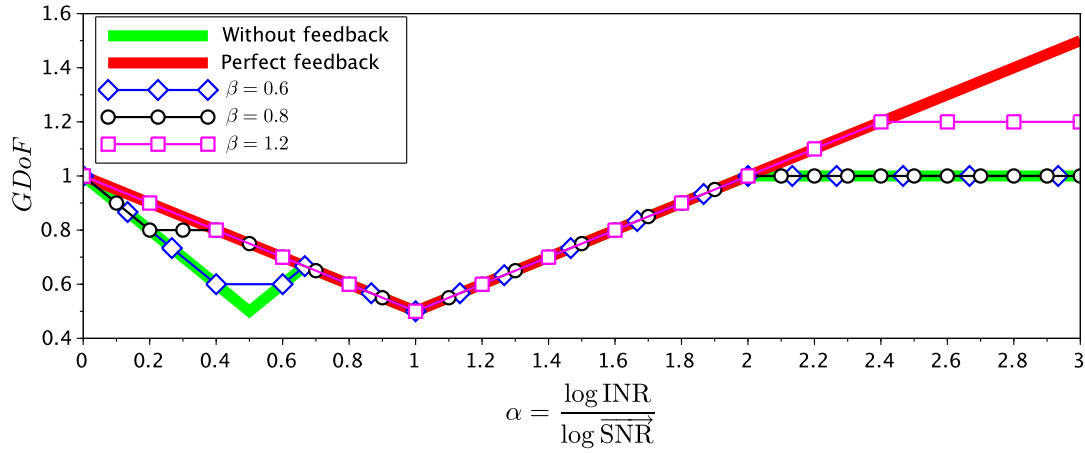
Figure 8: Generalized Degrees of Freedom (GDoF) as a function of parameters \alpha and \beta , with 0 \leq \alpha \leq 3 and \beta \in \{\frac{3}{5}, \frac{4}{5}, \frac{6}{5}\} , of the symmetric LD-IC-NOF. The plot without feedback is obtained from [8] and the plot with perfect-output feedback is obtained from [14].
