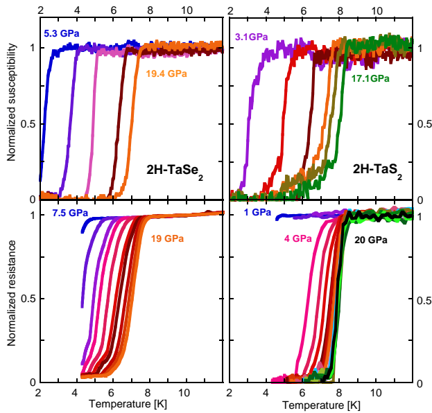
FIG. 1. Upper panels: Susceptibility of 2H-TaSe 2 (left panel) and 2H-TaS 2 (right panel) as a function of temperature for several applied pressures (5.3, 8.1, 11.7, 16.7 and 19.4 GPa for 2H-TaSe 2 and 3.1, 5.8, 7.9, 9.8, 14.8 and 17.1 GPa for 2H-TaS 2 ). Susceptibility has been normalized to the value found at 10 K, and the low temperature value has been modified to give zero. Lower panels: Resistance as a function of temperature for 2H-TaSe 2 (left panel) and for 2H-TaS 2 (right panel) for several applied pressures (from 7.5 to 15 by 1.5 GPa step and then every GPa up to 19 GPa for 2H-TaSe 2 and every GPa from 1 to 20 GPa for 2H-TaS 2 ). The resistance has been normalized to its value at 10 K.
