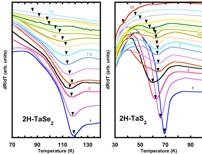
FIG. 2. Derivative of the resistance close to the CDW ordering temperature for respectively 2H-TaSe 2 (left panel) and 2H-TaS 2 (right panel) for different pressures (1, 2, 3, 4, 5, 6, 7.5, 9, 10.5, 12, 13.5, 15, 16, 17, 18 and 19 GPa (left) and every GPa from 1 to 17 GPa (right)). Curves are shifted in the y-axis for clarity. An arrow is used to mark the position where we take T_{CDW} to give the pressure dependence discussed in Fig 3.
