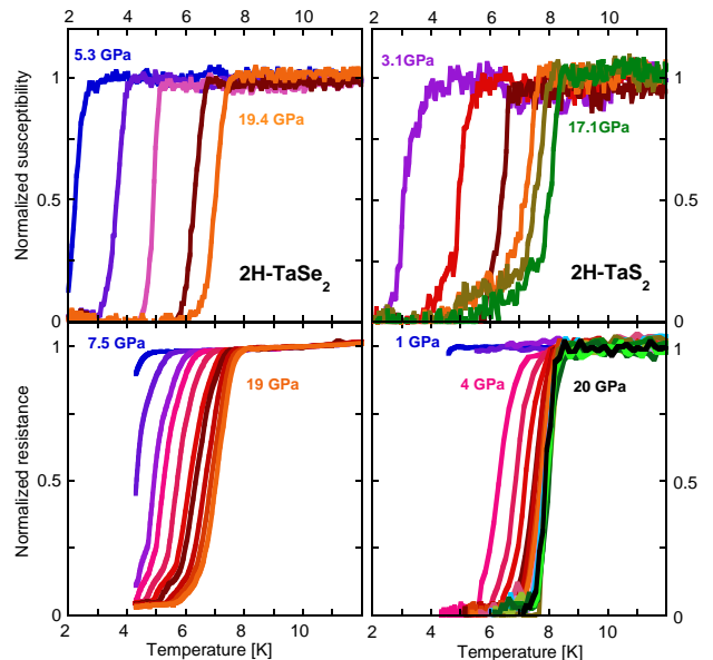
FIG. 1. Upper panels: Susceptibility of 2H-TaSe 2 (left panel) and 2H-TaS 2 (right panel) as a function of temperature for several applied pressures (5.3, 8.1 11.7 16.7 and 19.4 GPa for 2H-TaSe 2 and 3.1 5.8 7.9 9.8 14.8 and 17.1 GPa for 2H-TaS 2 ). Susceptibility has been normalized to the value found at 10 K, and the low temperature value has been modified to give zero. Lower panels: Resistance as a function of temperature for 2H-TaSe 2 (left panel) and for 2H-TaS 2 (right panel) for several applied pressures (from 7.5 to 15 by 1.5 GPa step and then every GPa up to 19 GPa for 2H-TaSe 2 and every GPa from 1 to 20 GPa for 2H-TaS 2 ). The resistance has been normalized to its value at 10 K.
