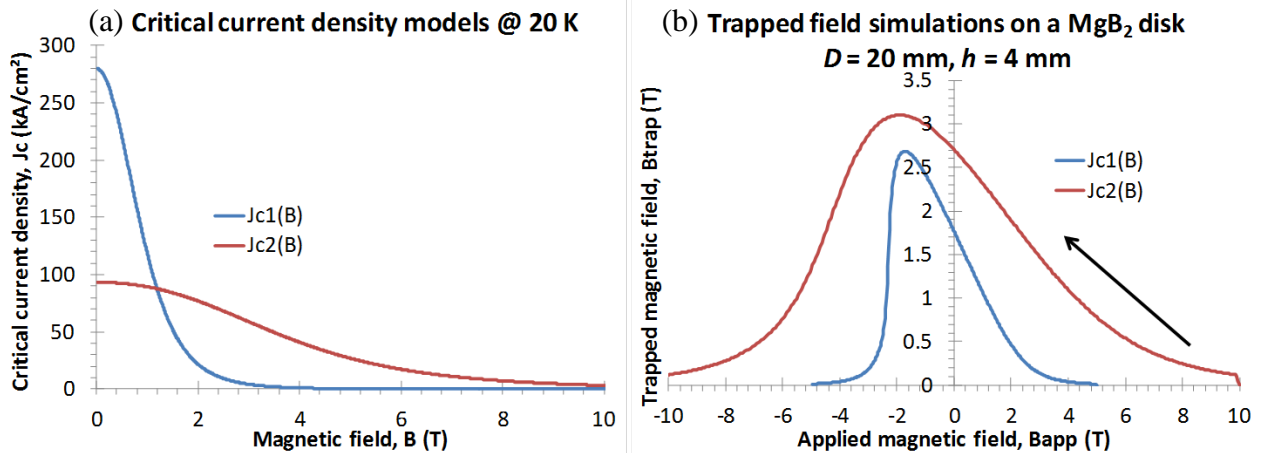
Fig. 1: Two models of critical current density (a), and the simulated resulting trapped magnetic field at the center of the surface of a bulk MgB 2 of 20 mm of diameter and 4 mm high (b).
