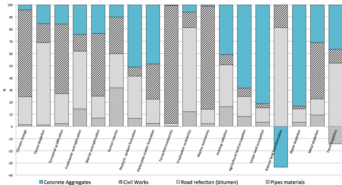
Figure 5: Breakdown of sewer infrastructure construction using ReCiPe V1.07 midpoint indicators
