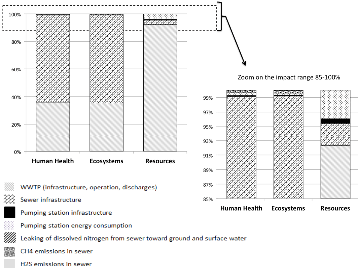
Figure 7: - Life Cycle Impact Assessment (LCIA) using ReCiPe Endpoint (H) V1.07 H2S / World ReCiPe H/H for the city of Grabels urban WWT system (sewer + WWTP)
