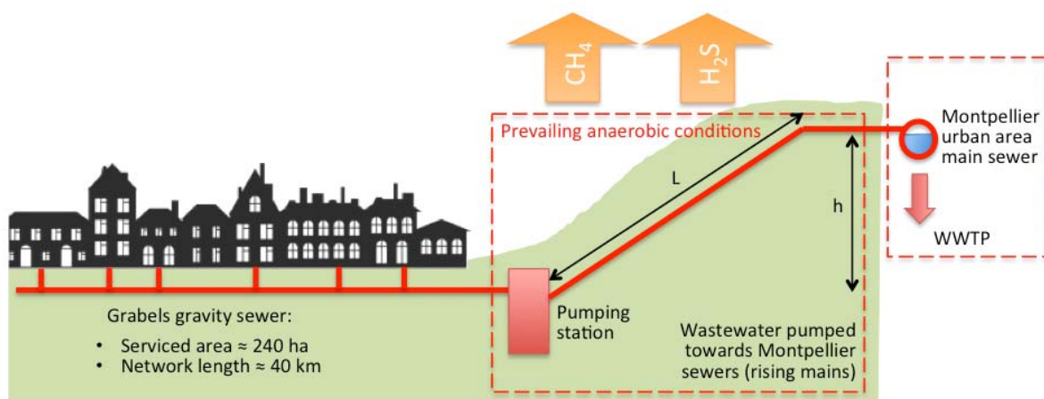
Figure 3: Sewer model of the serviced area of Grabels, France
