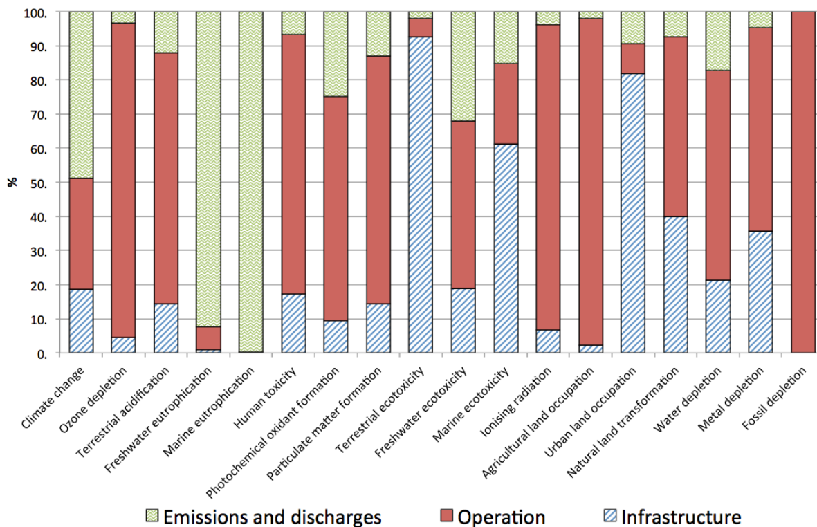
Figure 6: Breakdown of the WWTP model using ReCiPe V1.07 midpoint indicator
