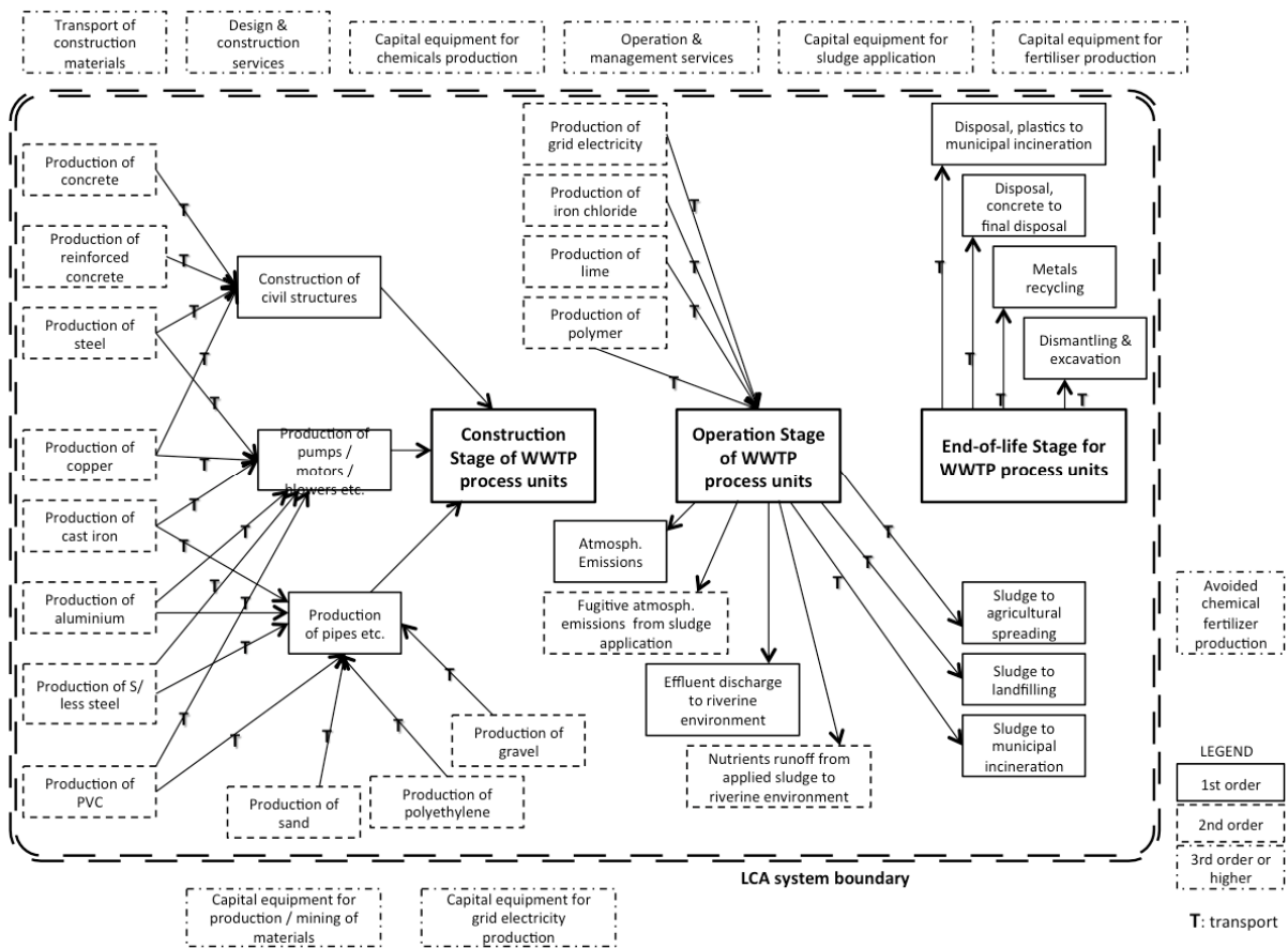
Figure 2: System boundary for life cycle inventory of WWTP
