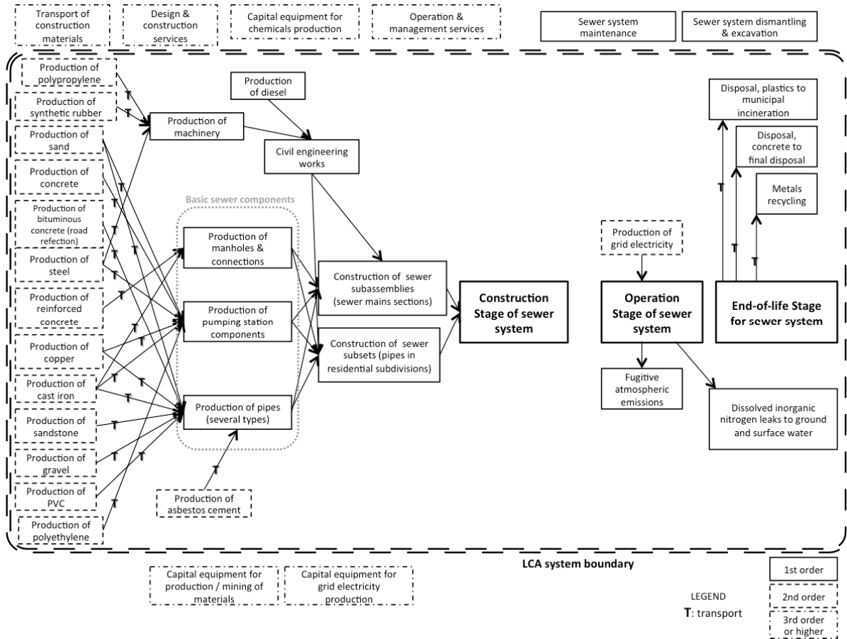
Figure 1: System boundary for life cycle inventory of sewer system
