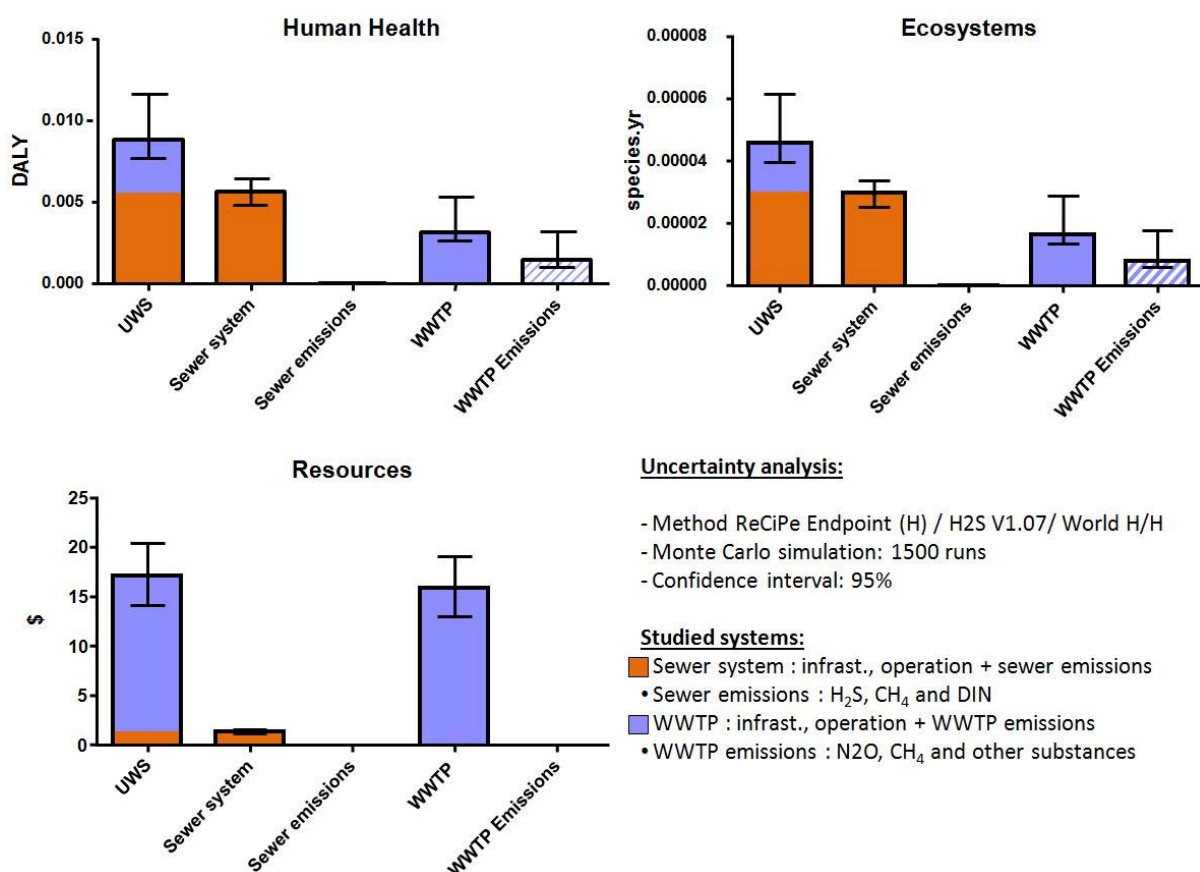
Figure 8: End-point indicators uncertainty assessment results (confidence interval of 95%) for the main components of the urban water system
