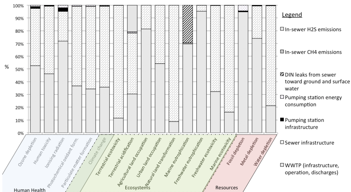
Figure 4: Life Cycle Impact Assessment (LCIA) using ReCiPe V1.07 midpoint indicators for the Grabels urban WWT system (sewer + WWTP)
