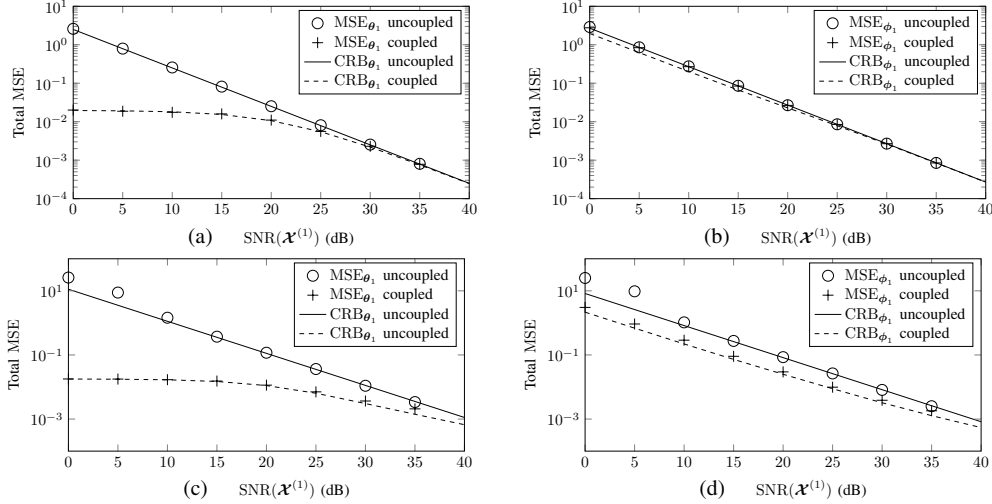
Fig. 1. Total mean squared error and performance bounds for the estimation of complex coupled CP tensor models. Uncoupled parameters \phi_{1:2} are vectorized real and imaginary parts of \mathbf{A}^{(1:2)} and \mathbf{B}^{(1:2)} , while coupled parameters (equality constraint) \theta_{1:2} are vectorized real and imaginary parts of \mathbf{C}^{(1:2)} . SNR of \mathcal{X}^{(2)} is fixed to 20dB whereas SNR( \mathcal{X}^{(1)} ) \in [0, 40] dB. Results for i.i.d. distributed \mathbf{A}^{(1)} are shown in (a) and (b), and for \mathbf{A}^{(1)} with two collinear columns are shown in (c) and (d).
