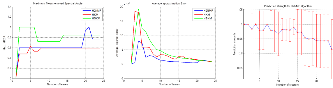
Figure 4: Left: the variation of the maximum MMSA (mean-removed spectral angle) to evaluate the homogeneity of clusters in terms of endmember signature. This is evaluated across the three hierarchical clustering algorithms: H2NMF, HSKM, HKM. We observe that all the three algorithms provide satisfactory results. Center: figure also shows the variation approximation error in equation (2) with increasing leaves for three hierarchical clustering algorithms. Right: Plot demonstrating the mean prediction strength calculated using the NMF decomposition. The red bars show the variance of the prediction strength. Optimal clusters are chosen based on the maximum of the prediction strength. Here for example it is 14.
