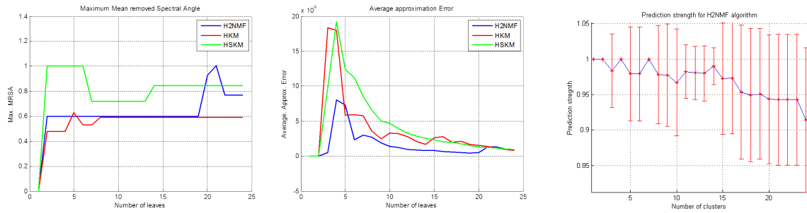
Figure 4: Left: the variation of the maximum MRSa (mean-removed spectral angle) to evaluate the homogeneity of clusters in terms of endmember signature. This is evaluated across the three hierarchical clustering algorithms: H2NMF, HSKM, HKM. We observe that all the three algorithms provide satisfactory results. Center: figure also shows the variation approximation error in equation (2) with increasing leaves for three hierarchical clustering algorithms. Right: Plot demonstrating the mean prediction strength calculated using the NMF decomposition. The red bars show the variance of the prediction strength. Optimal clusters are chosen based on the maximum of the prediction strength. Here for example it is 14.
