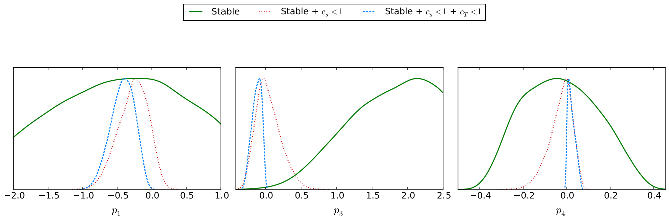
FIG. 3: Planck constraints on the 3D -model, the minimal EFT extension of the six-parameter \Lambda CDM model. The marginalised, posterior distribution for p_1 , p_3 and p_4 is shown. The likelihood analysis is carried out by also letting vary the six parameters of the standard \Lambda CDM model and the foreground parameters. The constraining power of theoretical priors is also shown: The solid line shows the posterior obtained after removing the portion of the parameter space in which unstable theories live. Likelihood intervals obtained by requiring that scalar perturbations, in stable theories, propagate at subluminal speed are shown by dotted lines. Dashed lines show results when also tensor perturbations are forced to propagate at subluminal speed.
