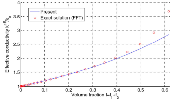
FIG. 3. (Color online) Comparison between present estimation [Eq. (16)] and exact solution (Fourier transform method with resolution 128 \times 128 \times 128 ). The microstructure is body-centered cubic with R_1 = 2R_2 , k_1 = 10k_0 , and k_2 = 0.1k_0 . The maximal volume fraction is 0.62 when the spheres touch each other.
