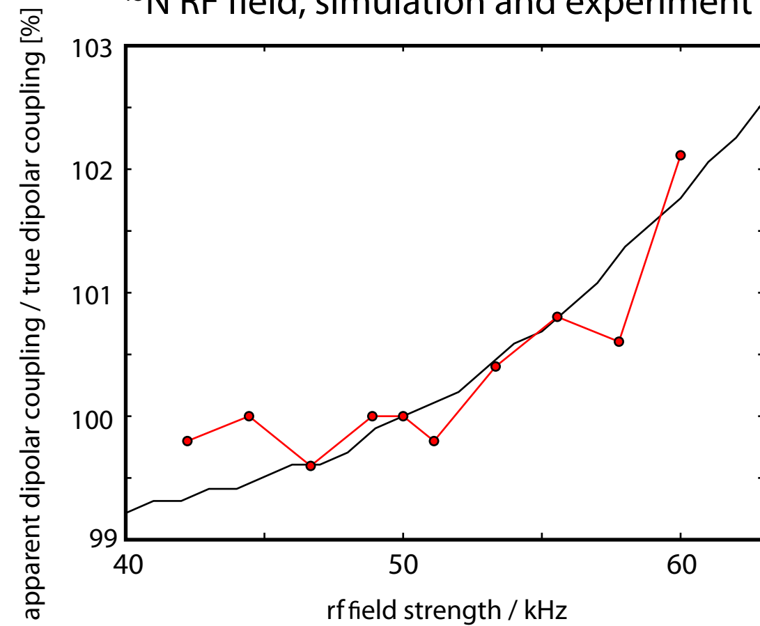
^{15}\text{N} RF field, simulation and experiment
