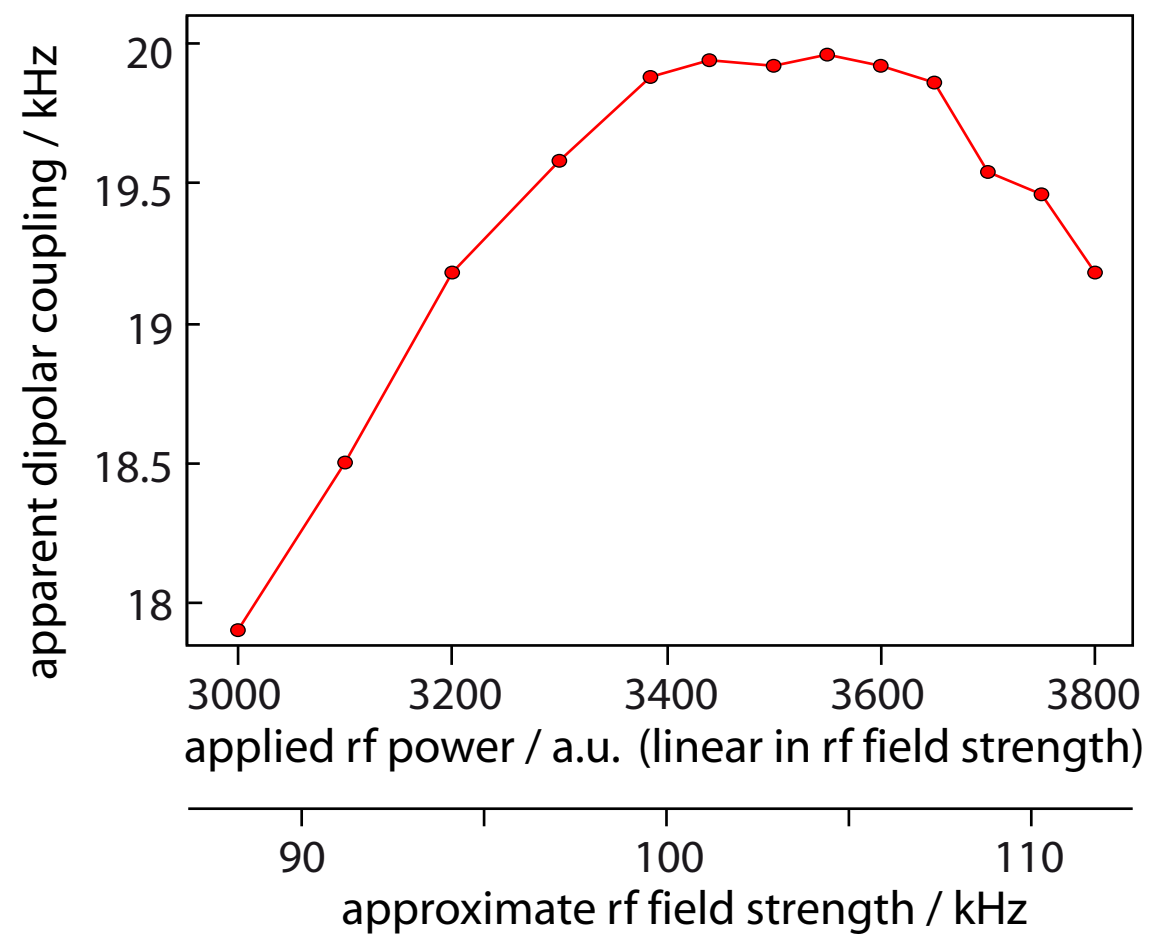
^1\text{H} RF field, experiment
