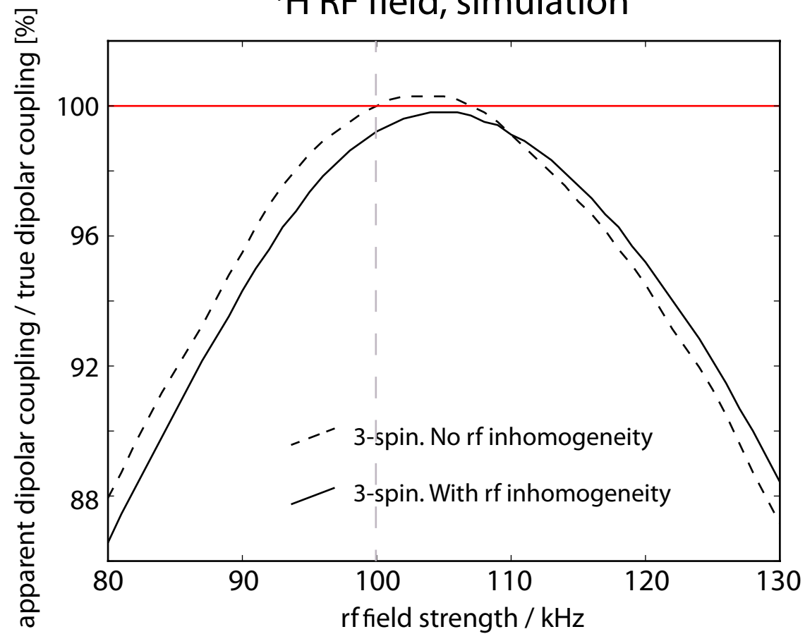
^1\text{H} RF field, simulation
