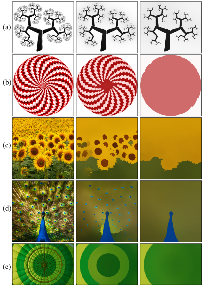
Fig. 13. Examples of the scale-space representation (center and right) of (left) input images. Scale-space is constructed by the SD filter ( u^0 = u_{l_1} ) with varying the regularization parameter \lambda : (a) 3 \times 10^2, 3 \times 10^3 , (b) 5 \times 10^3, 5 \times 10^5 , (c) 1 \times 10^3, 5 \times 10^3 , (d) 1 \times 10^3, 1 \times 10^4 , (e) 3 \times 10^3, 1 \times 10^4 .
