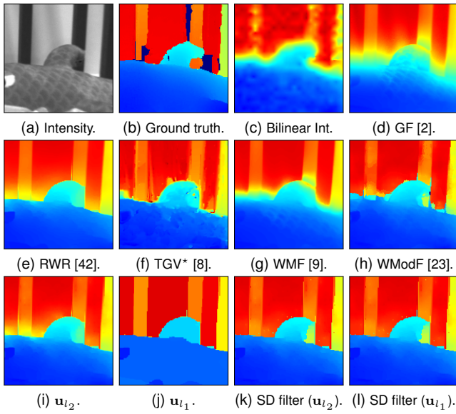
Fig. 11. Visual comparison of upsampled depth images on a snippet of the shark sequence in the Graz dataset [8]: (a) a high-resolution intensity image, (b) a ground-truth depth image, (c) bilinear interpolation, (d) GF [2], (e) RWR [42], (f) TGV* [8], (g) WMF [9], (h) WModF [23], (i) \mathbf{u}_{l_2} , (j) \mathbf{u}_{l_1} , (k) SD filter ( \mathbf{u}^0 = \mathbf{u}_{l_2} ), and (l) SD filter ( \mathbf{u}^0 = \mathbf{u}_{l_1} ). Note that the l_1 regularizer in (j) favors a piecewise constant solution, and this is problematic in a slanted surface. TGV* denotes the results provided by the authors of [8].
