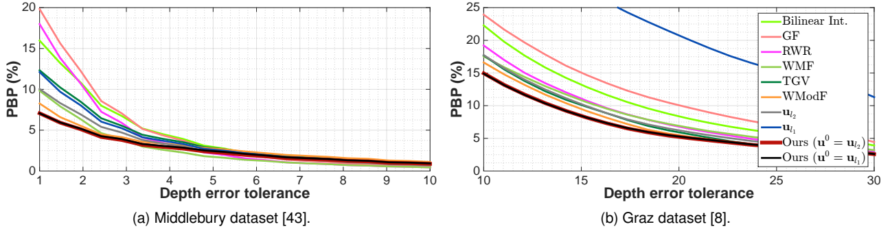
Fig. 7. Average PBP on (a) the Middlebury dataset [43] and (b) the Graz dataset [8] as a function of the depth error tolerance \delta . (Best viewed in colour.)
