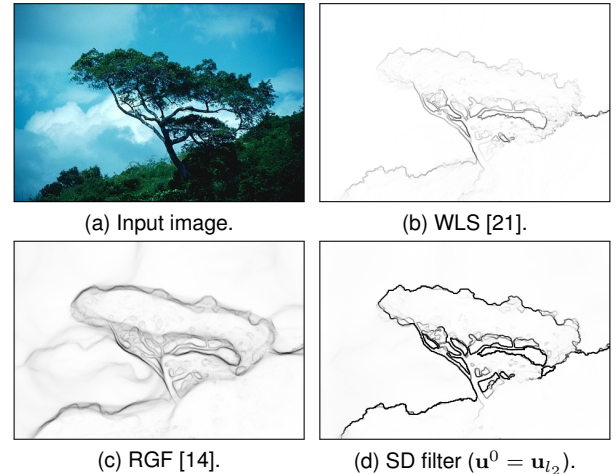
Fig. 15. Examples of the gradient magnitude averaged over scale-space: Given (a) an input image, scale-space is obtained by (b) WLS [21] ( \mu = 40 ), (c) RGF [14] ( \sigma_r = 0.05, k = 5 ), and (d) the SD filter ( \mathbf{u}^0 = \mathbf{u}_{l_2} ) with varying scale parameters. For each method, we set the maximum scale parameters manually, such that all the filtered images have similar smoothing levels. The gradient magnitude is then computed at each scale and averaged over scale-space.
