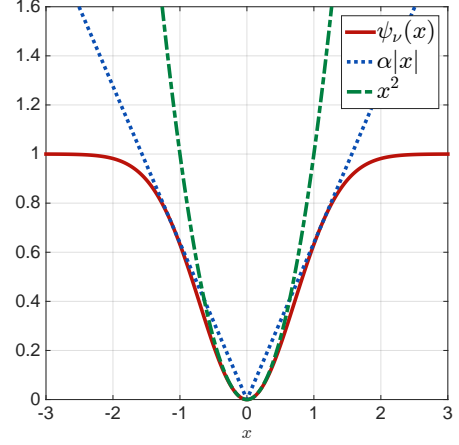
Fig. 5. Upper bounds on Welsch's function \psi_\nu : an l_2 regularizer x^2 and an l_1 regularizer \alpha|x| (a tight upper bound on \psi_\nu , when \nu is set to 1). (Best viewed in colour.)
