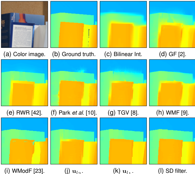
Fig. 8. Visual comparison of upsampled depth images on a snippet of the books sequence in the Middlebury dataset [43]: (a) a high-resolution color image, (b) a ground-truth depth image, (c) bilinear interpolation, (d) GF [2], (e) RWR [42], (f) Park et al. [10], (g) TGV [8], (h) WMF [9], (i) WModF [23], (j) u_{l_2} , (k) u_{l_1} , and (l) SD filter ( u^0 = u_{l_1} ). In contrast to the static guidance filters such as GF [2] and WMF [9], the SD filter interpolates the low-resolution depth image using the structure of both color and depth images, preserving sharp depth edges.
