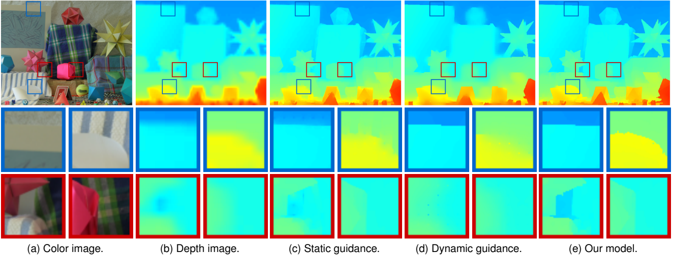
Fig. 2. Comparison of static and dynamic guidance filtering methods. Given (a) a high-resolution color image, (b) a low-resolution depth image is upsampled ( \times 8 ) by our model using (c) static guidance only, (d) dynamic guidance only, and (e) joint static and dynamic guidance. Static guidance filtering restores smoothed depth edges, as in the red boxes of (c). However, this method transfers all the structural information of the color image to the depth image, such as the weak color edges between the board and background and the color stripes on the tablecloth in the blue boxes of (c). Dynamic guidance filtering avoids this problem, as in the blue boxes of (d), but this method does not use the structural information of the high-resolution color image, smoothing or even eliminating depth edges as in the red boxes of (d). The SD filter jointly uses the structure of color and depth images, and does not suffer from these problems as in the blue and red boxes of (e). See Section 5.1 for details. (Best viewed in colour.)
