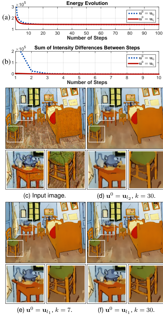
Fig. 6. Examples of (a) energy evolution and (b) a sum of intensity difference between successive steps (i.e., \|\mathbf{u}^k - \mathbf{u}^{k+1}\|_1 ), given (c) the input image. Our solver converges in fewer steps with the l_1 initialization ( \mathbf{u}^0 = \mathbf{u}_{l_1} ) than with the l_2 one ( \mathbf{u}^0 = \mathbf{u}_{l_2} ), with faster overall speed. It also guarantees a meaningful solution in the steady-state: (d) \mathbf{u}^0 = \mathbf{u}_{l_2} , k = 30 , (e) \mathbf{u}^0 = \mathbf{u}_{l_1} , k = 7 , and (f) \mathbf{u}^0 = \mathbf{u}_{l_1} , k = 30 . In this example, for removing textures, static guidance is set to the Gaussian filtered version (standard deviation, 1) of the input image ( \lambda = 50 , \mu = 5 , \nu = 40 ). See Section 5.2 for details.
