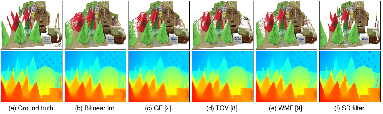
Fig. 9. Examples of (top) point cloud scene reconstruction using (bottom) depth images computed by (a) the ground truth, (b) bilinear interpolation, (c) GF [2], (d) TGV [8], (e) WMF [9], and (f) SD filter ( \mathbf{u}^0 = \mathbf{u}_{l_2} ). Current depth upsampling methods smooth depth edges, causing jagged artifacts.
