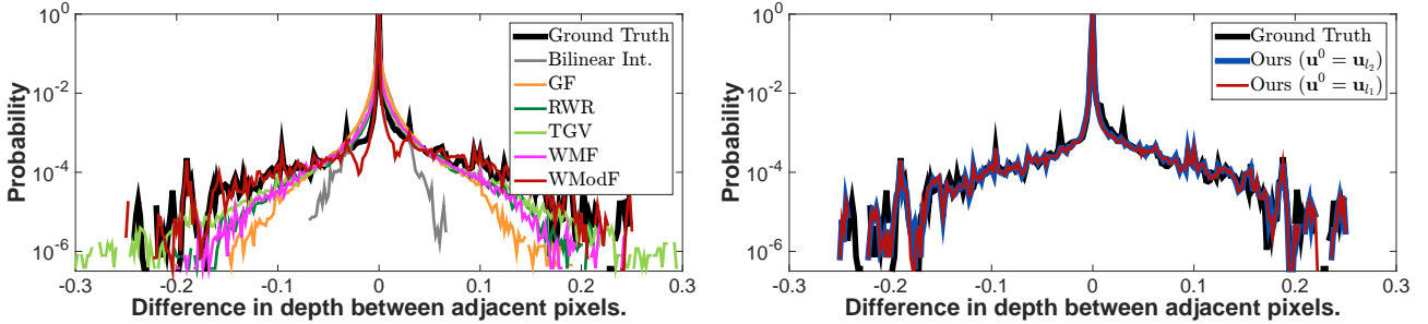
Fig. 10. \text{Log}_{10} of the normalized histograms (probability) of relative depths between adjacent pixels. Each histogram is computed using depth gradients along x- and y-axis, and then averaged on the Middlebury dataset [43]. (Best viewed in colour.)
