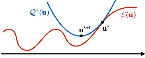
Fig. 3. Sketch of the majorization-minimization algorithm. At step k , a surrogate function Q^k is constructed given some estimate \mathbf{u}^k of the minimum of \mathcal{E} , such that Q^k(\mathbf{u}^k) = \mathcal{E}(\mathbf{u}^k) and Q^k(\mathbf{u}) \geq \mathcal{E}(\mathbf{u}) . At step k+1 , the next estimate \mathbf{u}^{k+1} is obtained by minimizing Q^k . These two steps are repeated until convergence.
