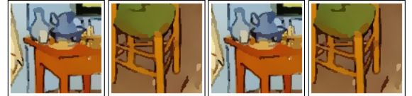
(e) \mathbf{u}^0 = \mathbf{u}_{l_1} , k = 7 .
