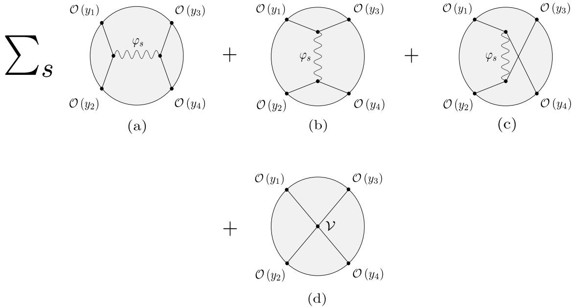
Figure 1: Four-point Witten diagrams contributing to the holographic reconstruction.
