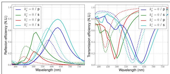
FIG. 18. Reflexion (left panel) and transmission (right panel) efficiencies of structure F2 obtained with the rigorous FEM calculation (line) and with the homogenization model (dashed).
