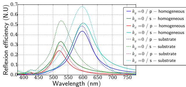
FIG. 19. (Dashed lines) Reflexion efficiency in the specular order for the structure F1 (same as left panel of Fig. 12). (Plain lines) Grating of silver nanocylinders of same dimensions as in optimized structure F1, but embedded in homogeneous \text{SiO}_2 background. Reflexion peaks in both panels are very similar.
