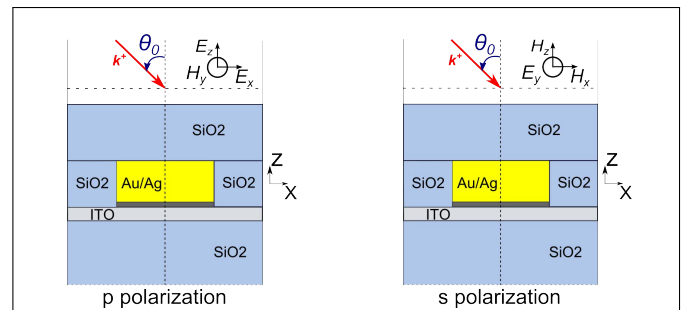
FIG. 2. Scheme of the illumination conditions for wavevector \mathbf{k}^+ lying in the xz -plane ( \psi_0 = 0 ).
