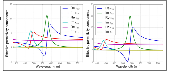
FIG. 16. Effective anisotropic relative permittivity components for the unit cell of structures F1 (left panel) and F2 (right panel).
