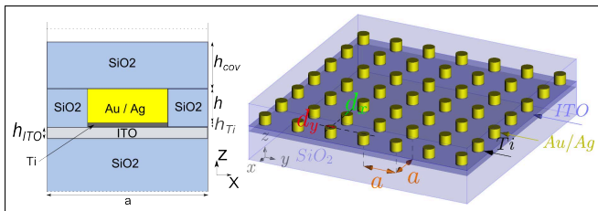
FIG. 1. Schemes of the considered nanoparticles gratings.
