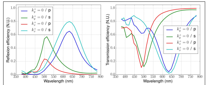
FIG. 13. Reflexion (left panel) and transmission (right panel) efficiencies in the specular order for the structure F2.
