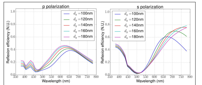
FIG. 7. Efficiency in the reflexion specular order for the group of structures S4.
