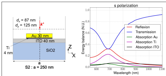
FIG. 8. Decomposition of the total energy balance for s-polarization for the structure S2.
