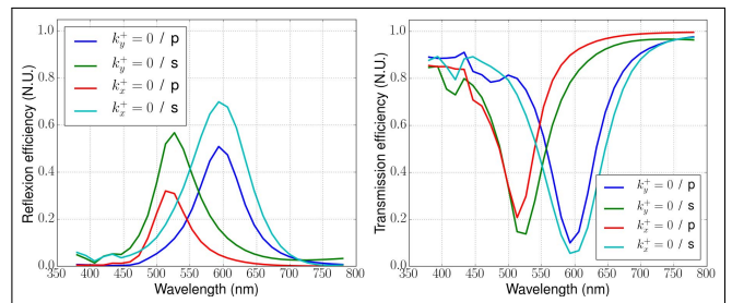
FIG. 12. Reflexion (left panel) and transmission (right panel) efficiencies in the specular order for the structure F1.
