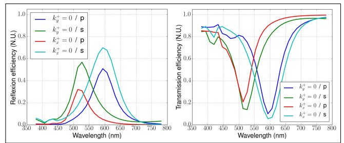
FIG. 12. Reflexion (left panel) and transmission (right panel) efficiencies in the specular order for the structure F1.
