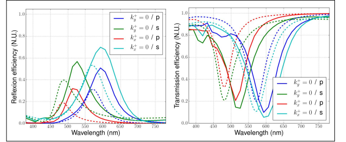
FIG. 17. Reflexion (left panel) and transmission (right panel) efficiencies of structure F1 obtained with the rigorous FEM calculation (line) and with the homogenization model (dashed).
