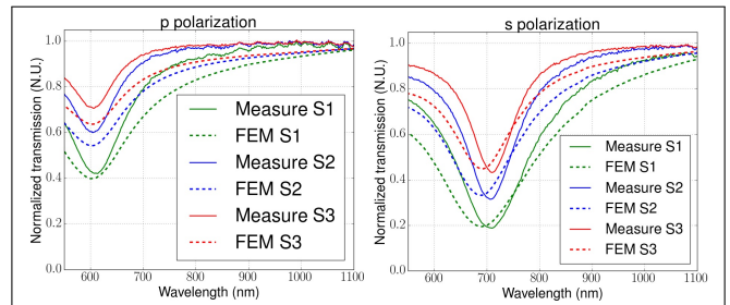
FIG. 4. Comparison between the FEM results (dashed) and the measurements (line) in transmission for the three fabricated samples S1–S2–S3 .
