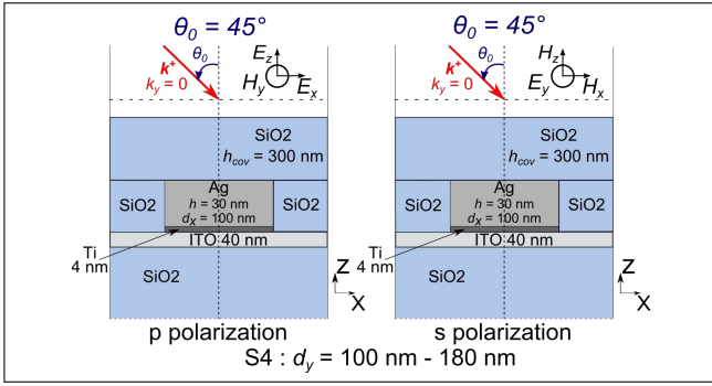
FIG. 5. Scheme of the structure S4 for the considered conditions of illumination.
