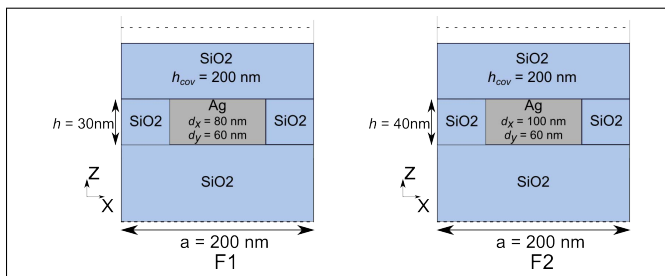
FIG. 11. Schemes of the optimized filters F1 (left panel) and F2 (right panel).
