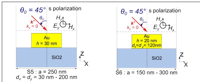
FIG. 9. Scheme of the structures S5 (left panel) and S6 (right panel).
