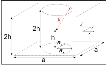
FIG. 15. Scheme of the considered unit cell.
