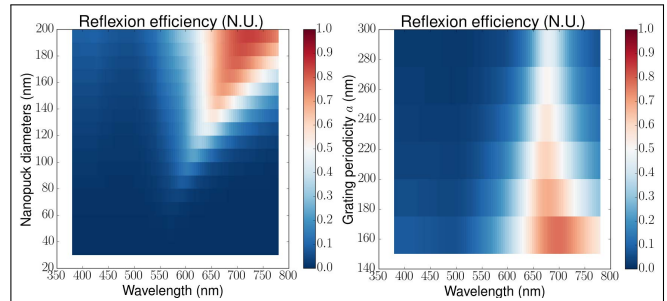
FIG. 10. Left panel: Reflexion efficiency in the specular order for structures S5. Right panel: Reflexion efficiency in the specular order for structures S6.
