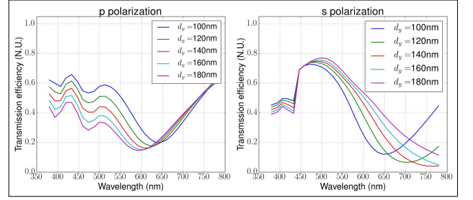
FIG. 6. Efficiency in the transmission specular order for the group of structures S4.
