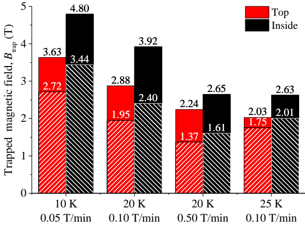
Fig. 7. Bar graph synthesizing the results of maximum trapped magnetic field using d20x2 . The hashed part of the bars represents the remanent trapped magnetic field B_{\text{rem}} , whereas the full bars are associated to the maximum trapped field B_{\text{trap}} .
