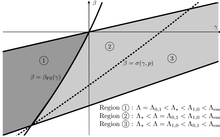
FIGURE 4. In the dark grey region, symmetry breaking occurs. The plot is done for p = 2 and d = 3 . See Appendix B for a more detailed description of the properties of the lowest eigenvalues.
