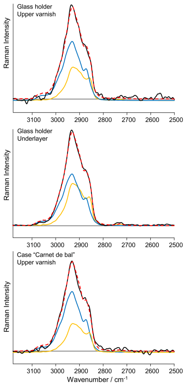
558 Fig. 7 : Spectral decomposition of FT-Raman CH band for three organic layers (mixtures) using linseed oil and 559 colophony films as pure reference materials. Misfitting examples are presented as supplementary data.
