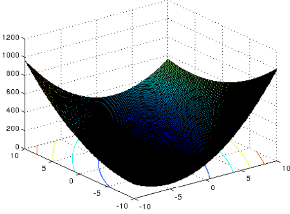
Fig. 1. Function x_p^o \mapsto \|\Psi_{qp}^{[s]}[x_p^o, u, w]\|_{RMS}^2 for u(t) = \sin(0.5t) , w_1(t) = \cos(-0.25 * t) and w_2(t) = 0
