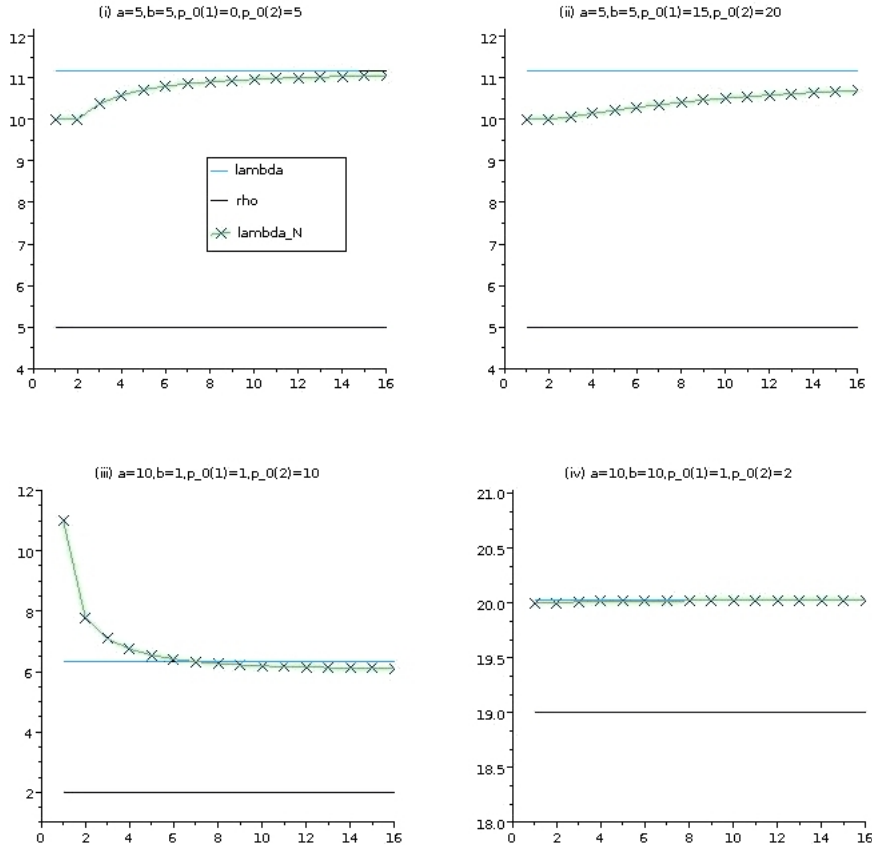
FIGURE 1. Evolution of the spectral gap with respect to the number of particles. Details are described in Subsection 3.5
