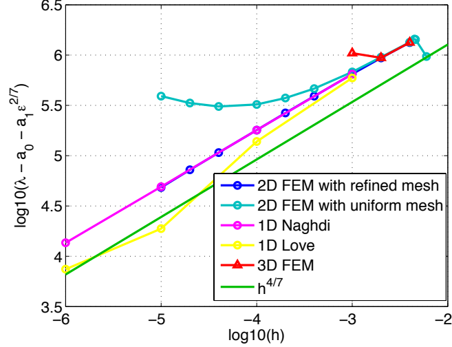
FIGURE 13. Shell (6.2)-(6.3): Computed values of \lambda_L(\varepsilon) - a_0 - a_1 \varepsilon^{2/7} versus thickness h = 2\varepsilon . 1D Naghdi and Love models in [2]. The reference line is h \mapsto \varepsilon^{4/7} E/\rho .
