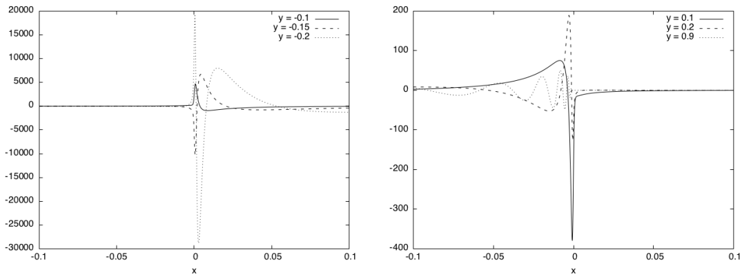
Figure 3: Real part of a singular manufactured solution F_1^{w,\nu} defined as in Figure 1 but with \delta(x, y) = 4y^2 + 1 to enhance the phase oscillations in the x direction close to the resonance x = 0 , a phenomenon that is reminiscent of some propagative singularities studied in [4]. Note that there are oscillations on both sides of the resonance, but because of the damping/growth phenomenon that occurs along y for x > 0 as discussed in Remark 17, they are visible on one side only.
