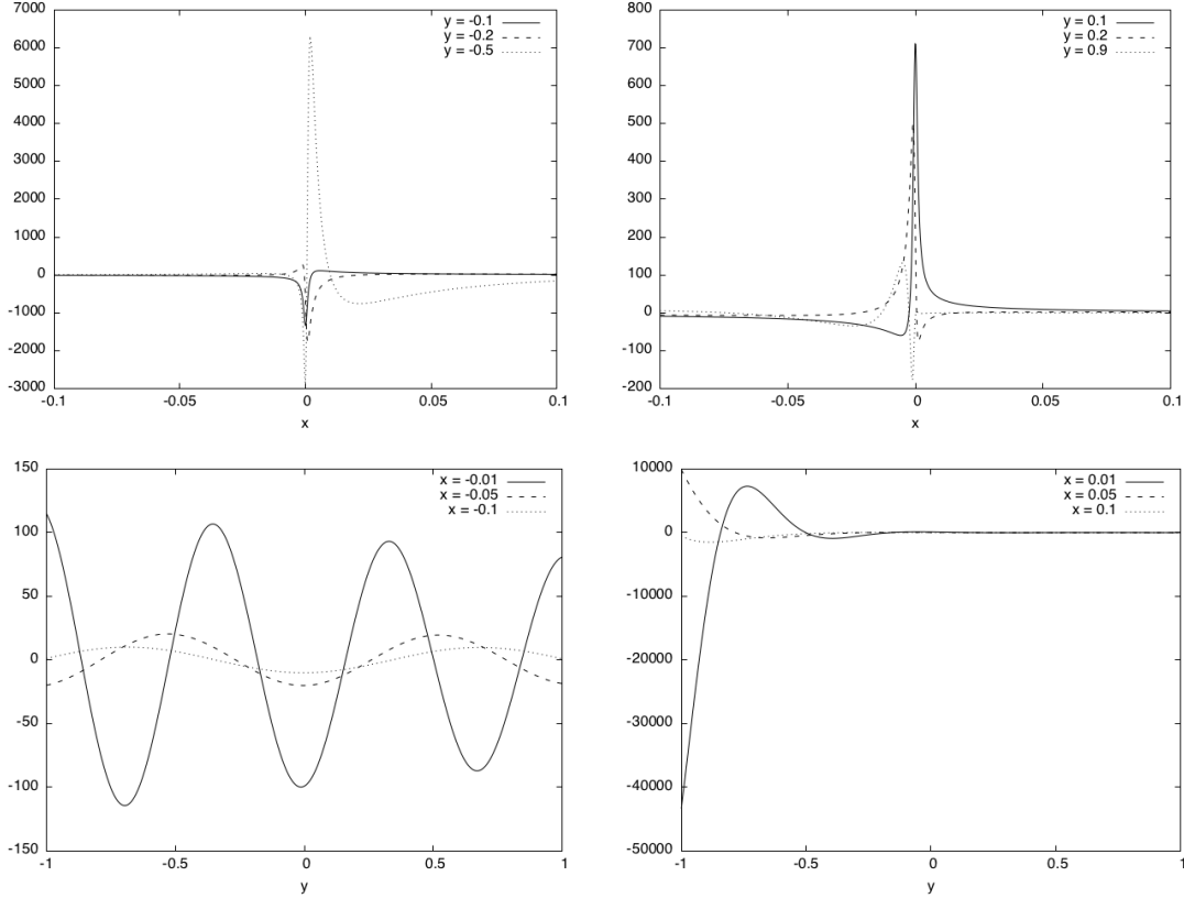
Figure 1: Real part of the singular manufactured solution F_1^{w,\nu} as given by (89) on a 2D domain \Omega = (-1, 1)^2 , with dissipation \nu = 0.001 and weight w \equiv 1 . Here the plasma-dependent parameters are \alpha(x, y) = -x and \delta(x, y) = y^2 + 1 . Upper plots show cuts in the x direction at specified values of y for y = -0.1 , y = -0.2 and y = -0.5 on the left and y = 0.1 , y = 0.2 and y = 0.9 on the right. Lower plots show cuts in the y direction at specified values of x , for x = -0.01 , x = -0.05 and x = -0.1 on the left and x = 0.01 , x = 0.05 and x = 0.1 on the right. The cuts x = 0 or y = 0 do not bring additional material so are not represented: they can be identified directly on Figure 2.
