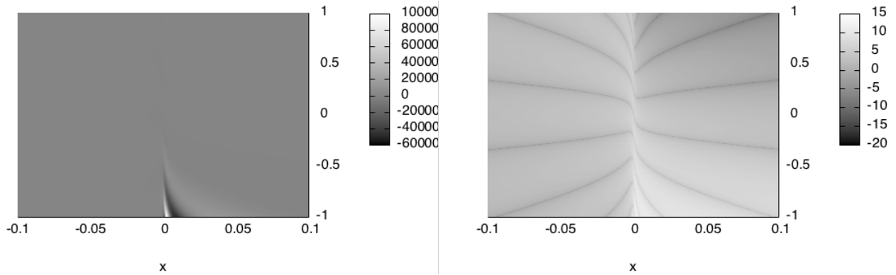
Figure 2: Real part of the singular manufactured solution F_1^{w,\nu} as given by (89) on a 2D domain \Omega = (-1, 1)^2 , with dissipation \nu = 0.001 and weight w \equiv 1 . As in Figure 1 above, the plasma-dependent parameters are \alpha(x, y) = -x and \delta(x, y) = y^2 + 1 . The right plot shows the same function in logscale, to improve the visibility of the oscillations along y outside the bottom-lower region where the negative sign of \sigma'(y) := \partial_y \delta(y, 0) creates an exponential growths in the -y direction, see Remark 17.
