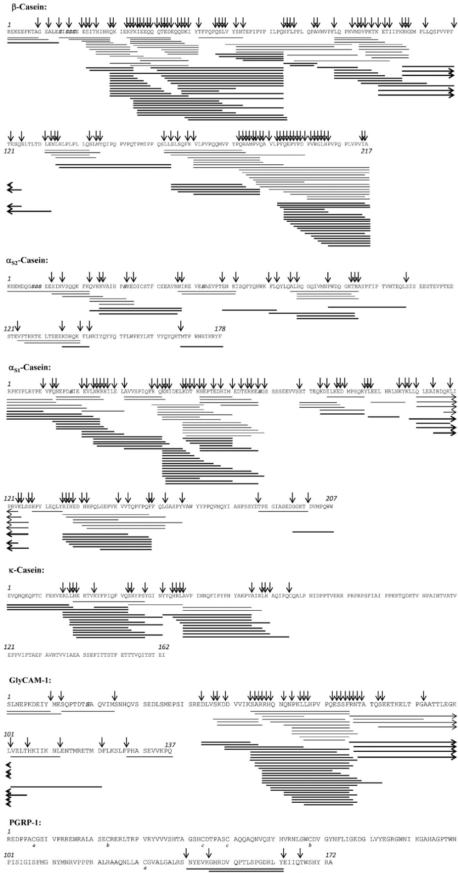
Fig. 2. Position of cleavage sites (vertical arrows) on the amino acid sequences of b-casein (Swiss-Prot accession number Q9TVD0), \alpha_{S2} -casein (O97944), \alpha_{S1} -casein (O97943), \kappa -casein (P79139), GlyCAM-1 (P15522) and PGRP-1 (Q9GK12), and location of peptides released during fermentation of camel milk by S. thermophilus LMD-9.
