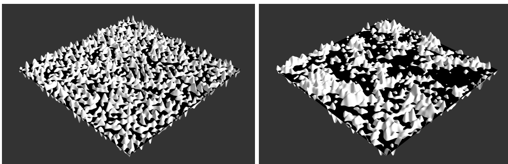
An instance of the cut-off field (resp. the COGFF) on the left (resp. right) on the flat torus with L = 1000 . The field is colored in white and the black surface is a
